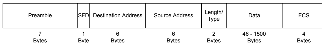
Figure 17-3. Ethernet Frame
