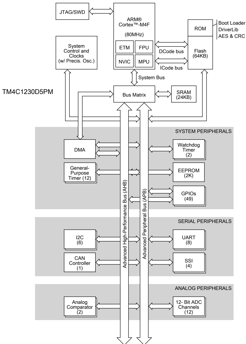
Figure 1-2. Tiva TM4C1230D5PM Microcontroller High-Level Block Diagram
