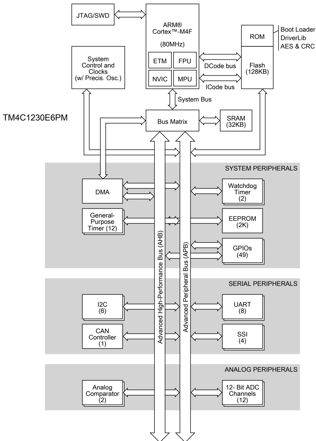
Figure 1-2. Tiva TM4C1230E6PM Microcontroller High-Level Block Diagram
