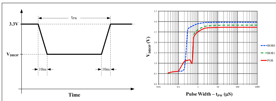
Figure 20-8. POR-BOR0-BOR1 VDD Droop Response
