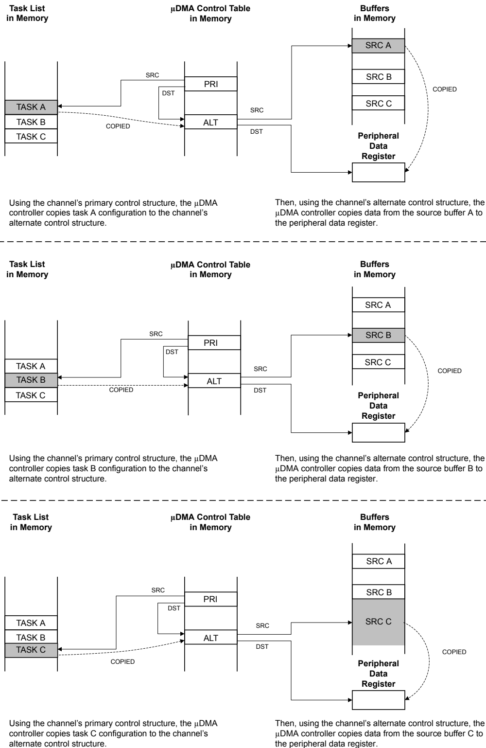
Figure 8-6. Peripheral Scatter-Gather, \mu DMA Copy Sequence
