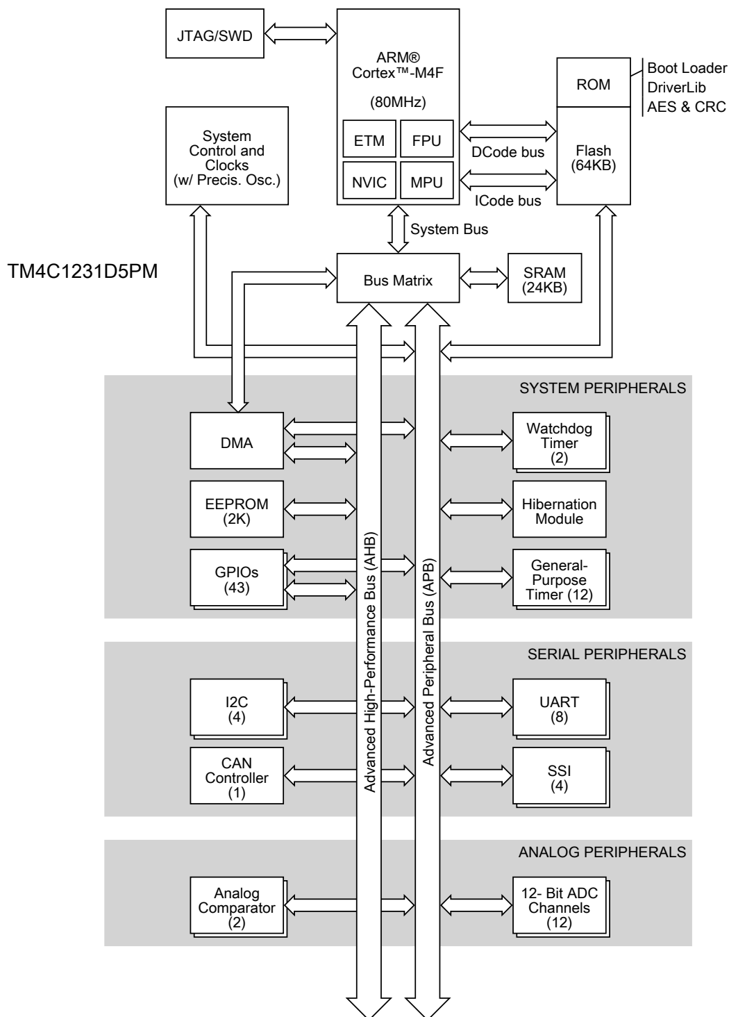
Figure 1-2. Tiva TM4C1231D5PM Microcontroller High-Level Block Diagram
