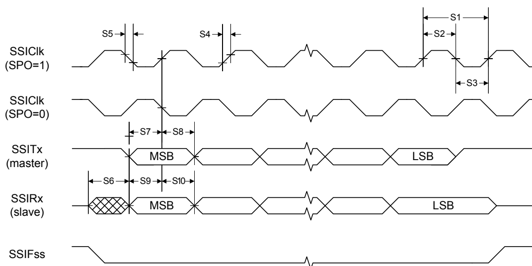
Figure 21-22. SSI Timing for SPI Frame Format (FRF=00), with SPH=1
