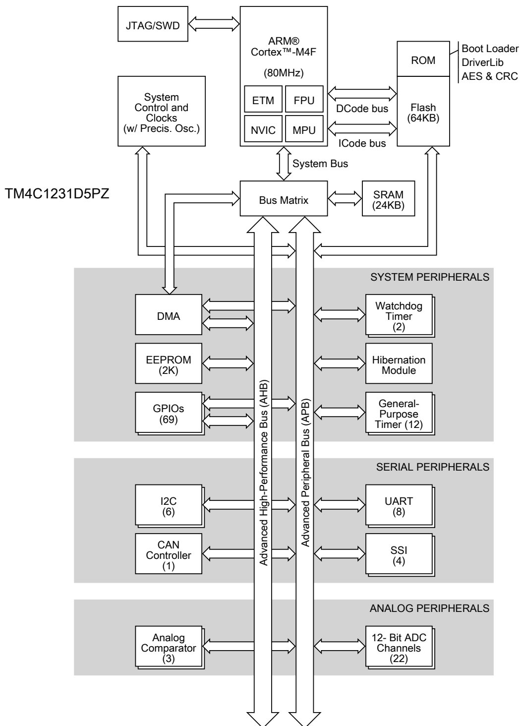
Figure 1-2. Tiva TM4C1231D5PZ Microcontroller High-Level Block Diagram
