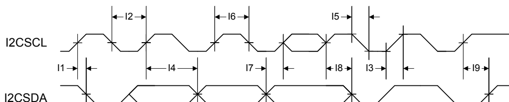
Figure 21-23. I 2 C Timing
