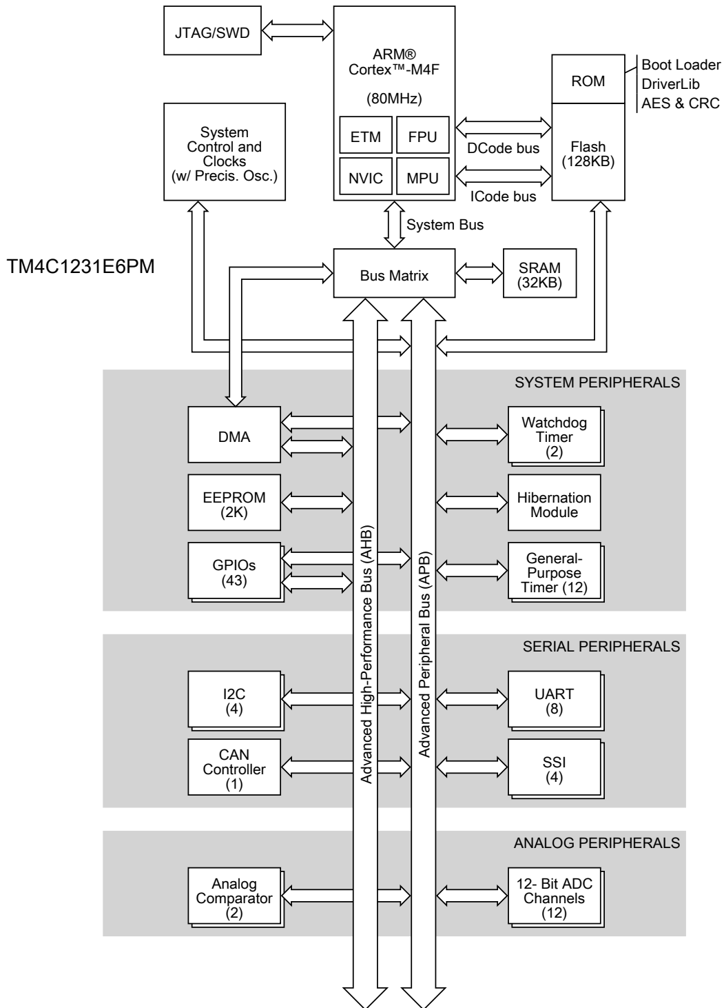
Figure 1-2. Tiva TM4C1231E6PM Microcontroller High-Level Block Diagram
