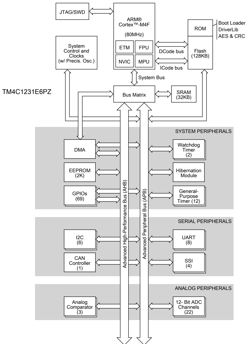
Figure 1-2. Tiva TM4C1231E6PZ Microcontroller High-Level Block Diagram
