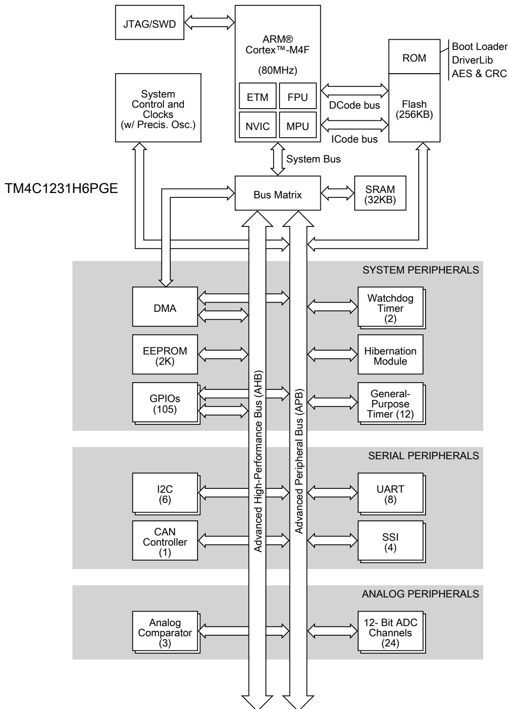
Figure 1-2. Tiva TM4C1231H6PGE Microcontroller High-Level Block Diagram
