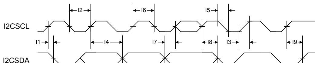
Figure 21-22. I 2 C Timing
