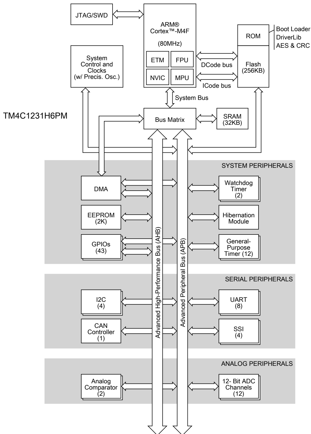
Figure 1-2. Tiva TM4C1231H6PM Microcontroller High-Level Block Diagram
