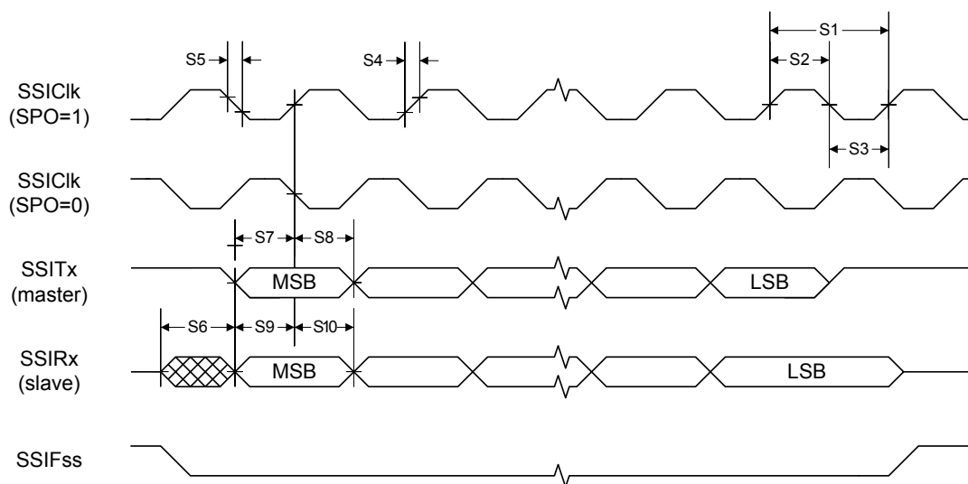
Figure 21-21. SSI Timing for SPI Frame Format (FRF=00), with SPH=1
