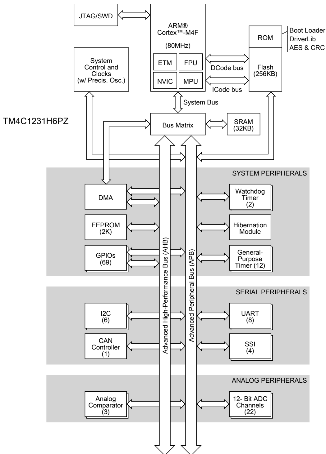
Figure 1-2. Tiva TM4C1231H6PZ Microcontroller High-Level Block Diagram
