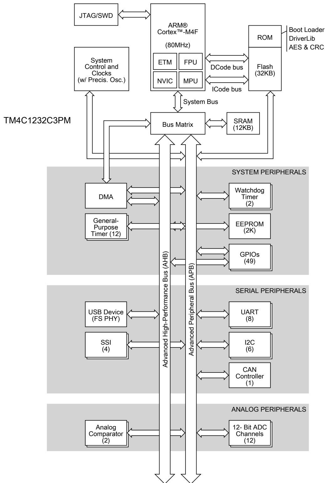
Figure 1-2. Tiva TM4C1232C3PM Microcontroller High-Level Block Diagram
