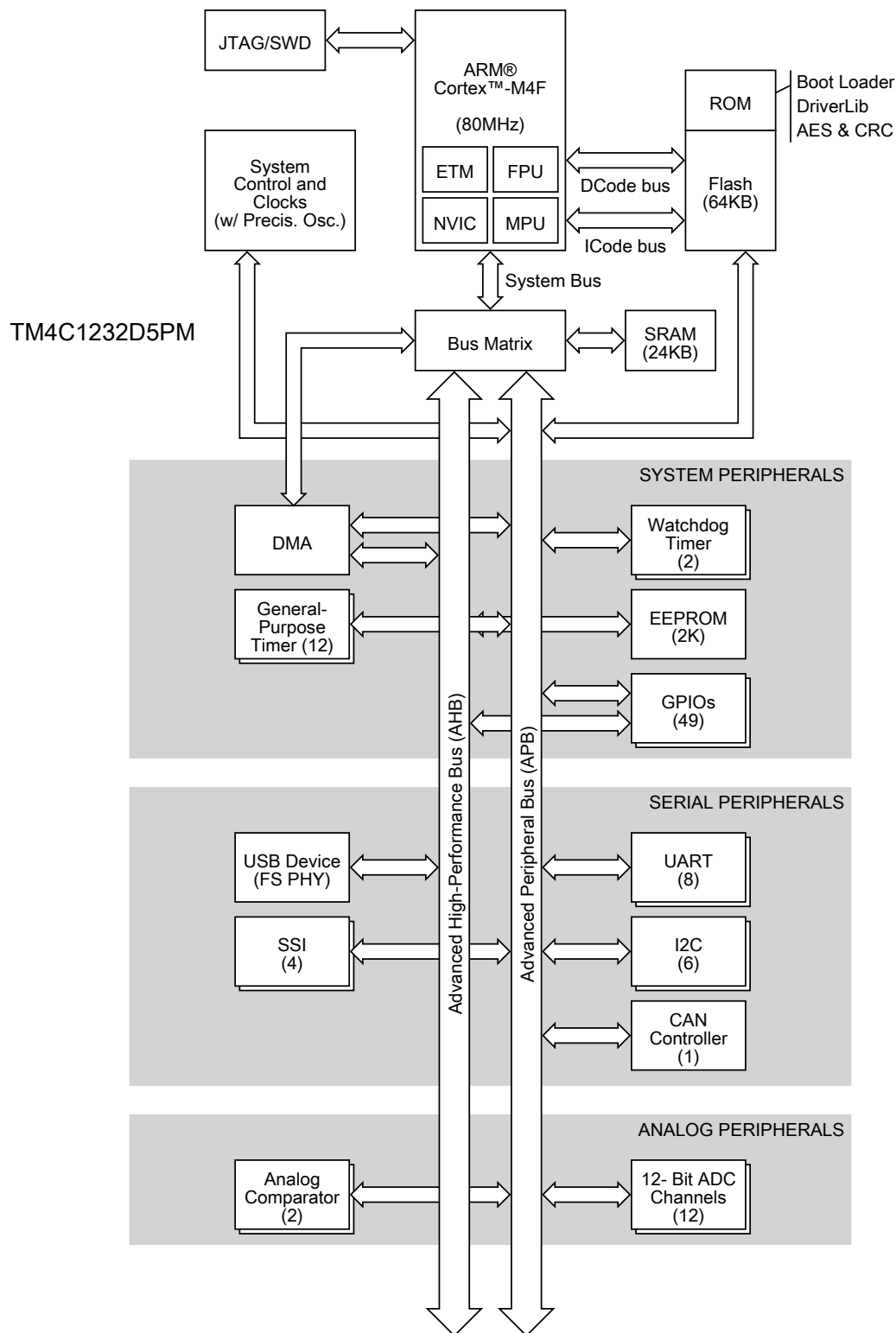
Figure 1-2. Tiva TM4C1232D5PM Microcontroller High-Level Block Diagram
