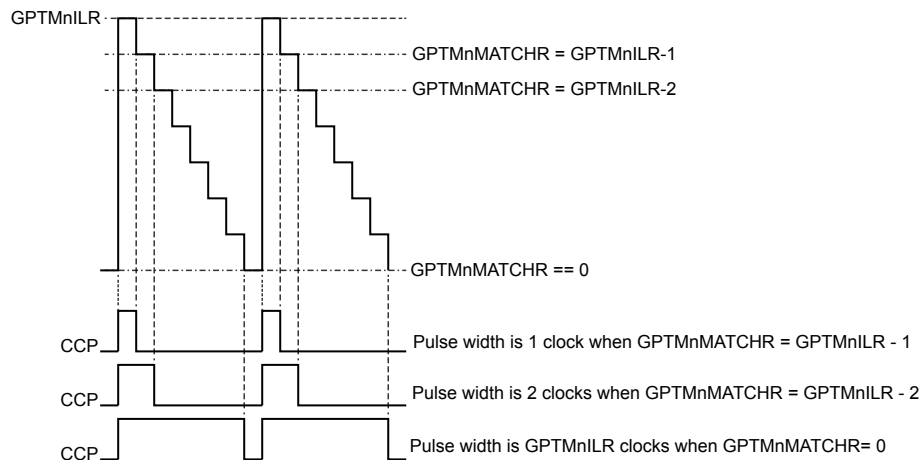
Figure 10-8. CCP Output, \text{GPTMTnILR} > \text{GPTMTnMATCHR}
