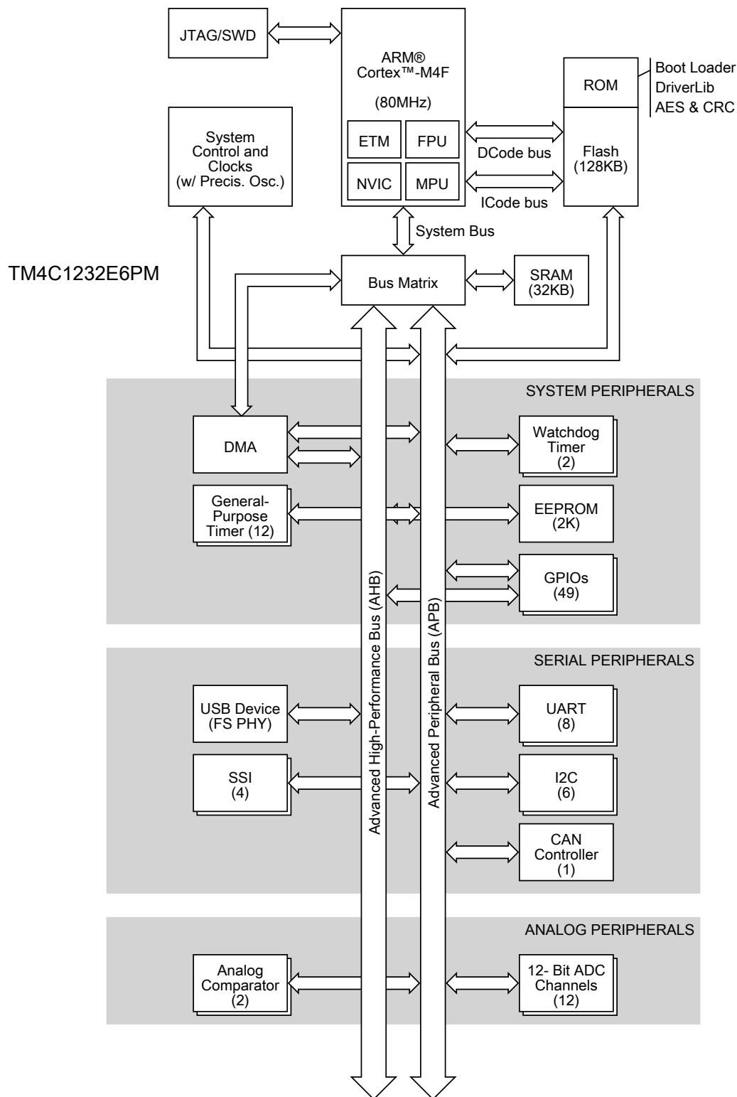
Figure 1-2. Tiva TM4C1232E6PM Microcontroller High-Level Block Diagram
