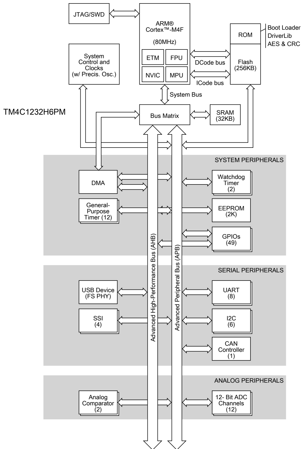
Figure 1-2. Tiva TM4C1232H6PM Microcontroller High-Level Block Diagram
