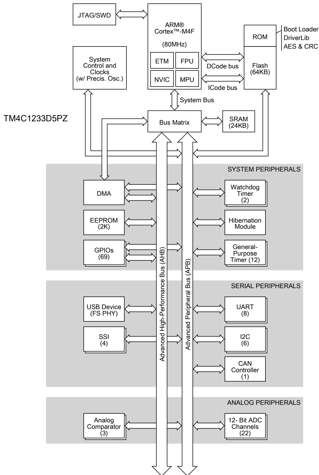
Figure 1-2. Tiva TM4C1233D5PZ Microcontroller High-Level Block Diagram
