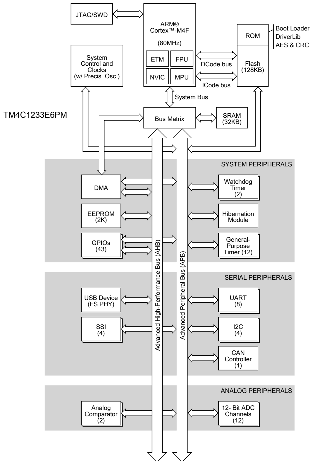
Figure 1-2. Tiva TM4C1233E6PM Microcontroller High-Level Block Diagram
