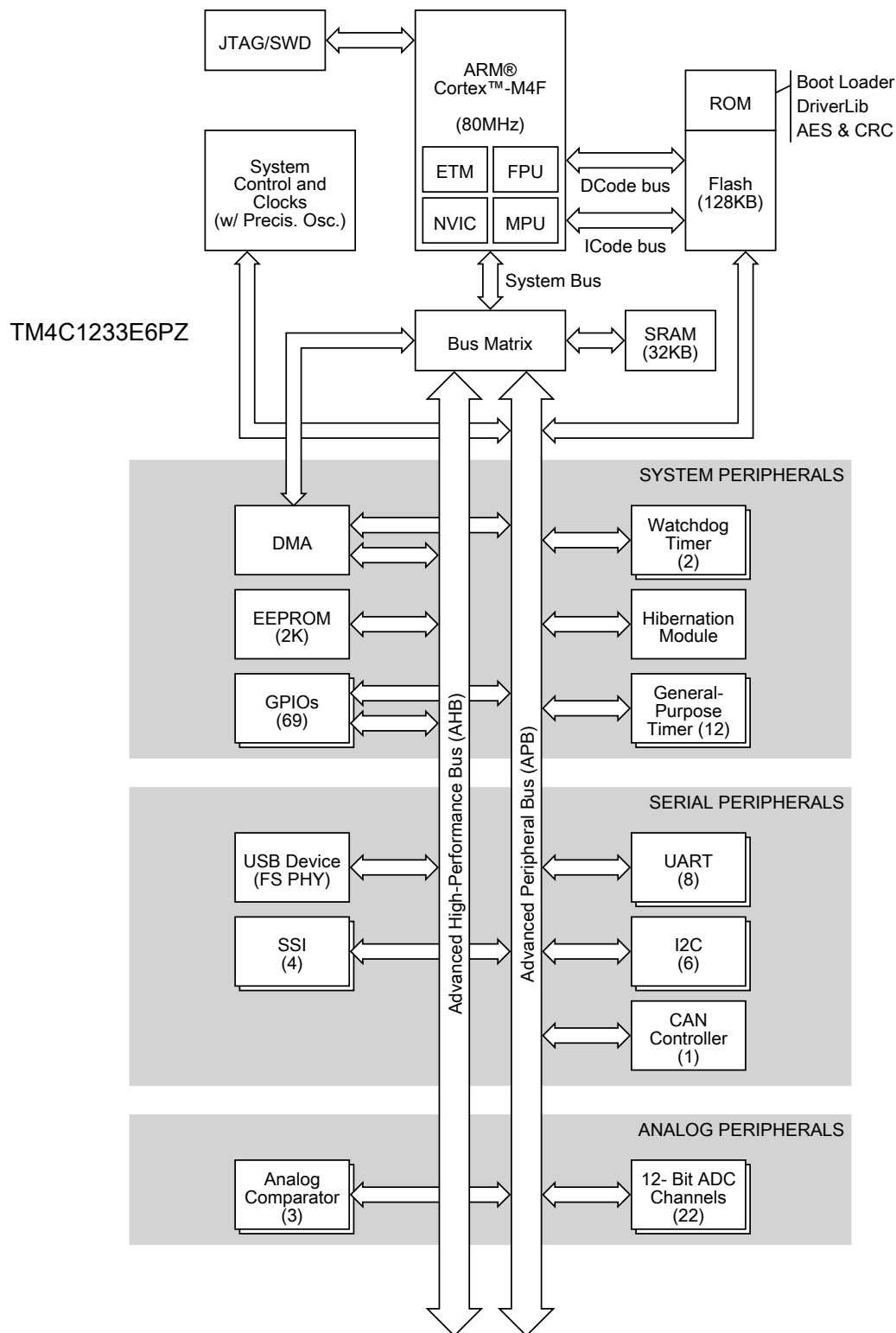
Figure 1-2. Tiva TM4C1233E6PZ Microcontroller High-Level Block Diagram
