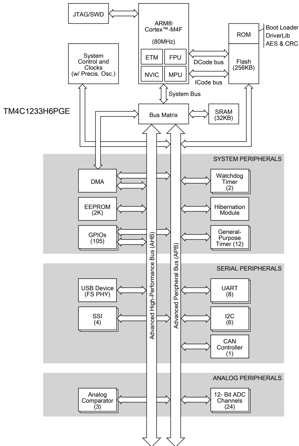
Figure 1-2. Tiva TM4C1233H6PGE Microcontroller High-Level Block Diagram
