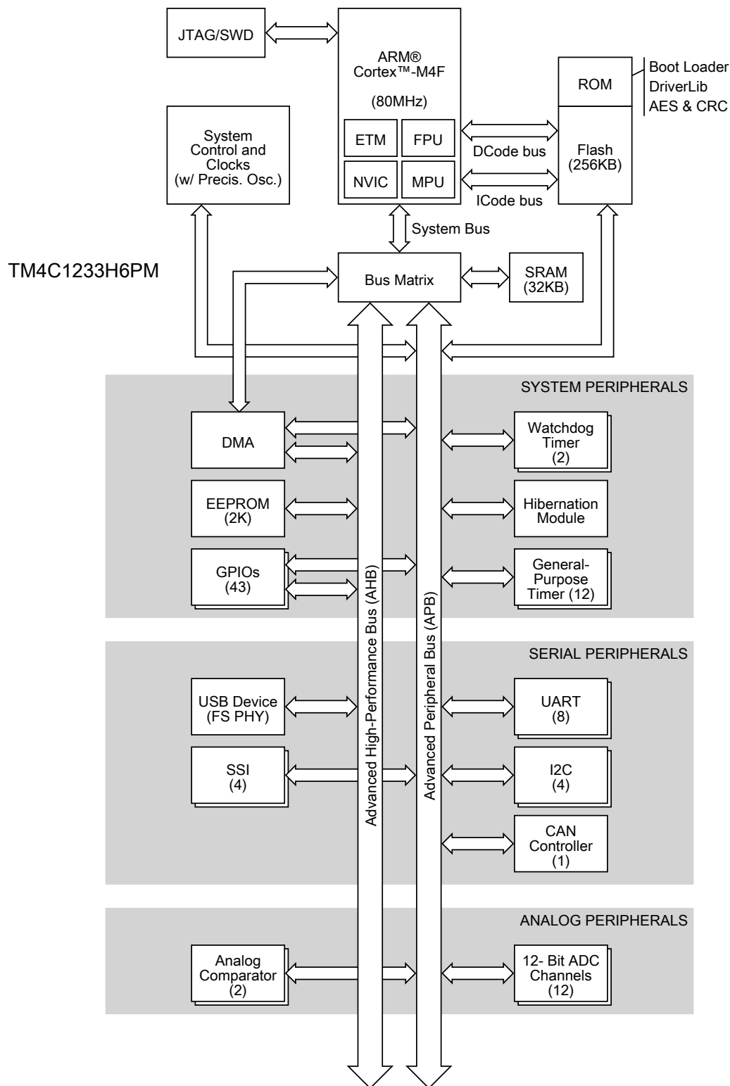
Figure 1-2. Tiva TM4C1233H6PM Microcontroller High-Level Block Diagram
