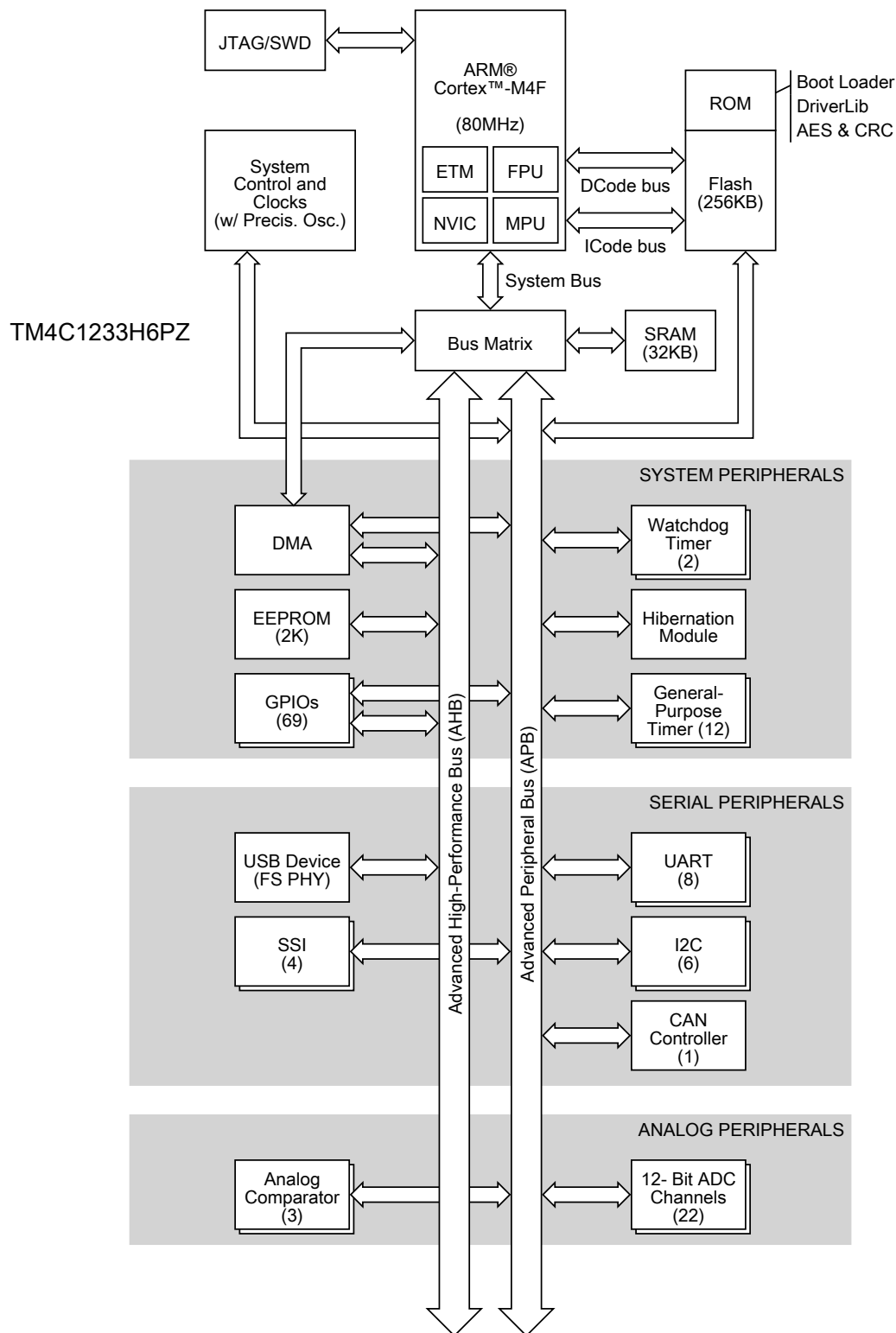
Figure 1-2. Tiva TM4C1233H6PZ Microcontroller High-Level Block Diagram
