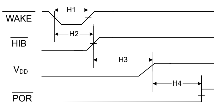
Figure 22-15. Hibernation Module Timing
