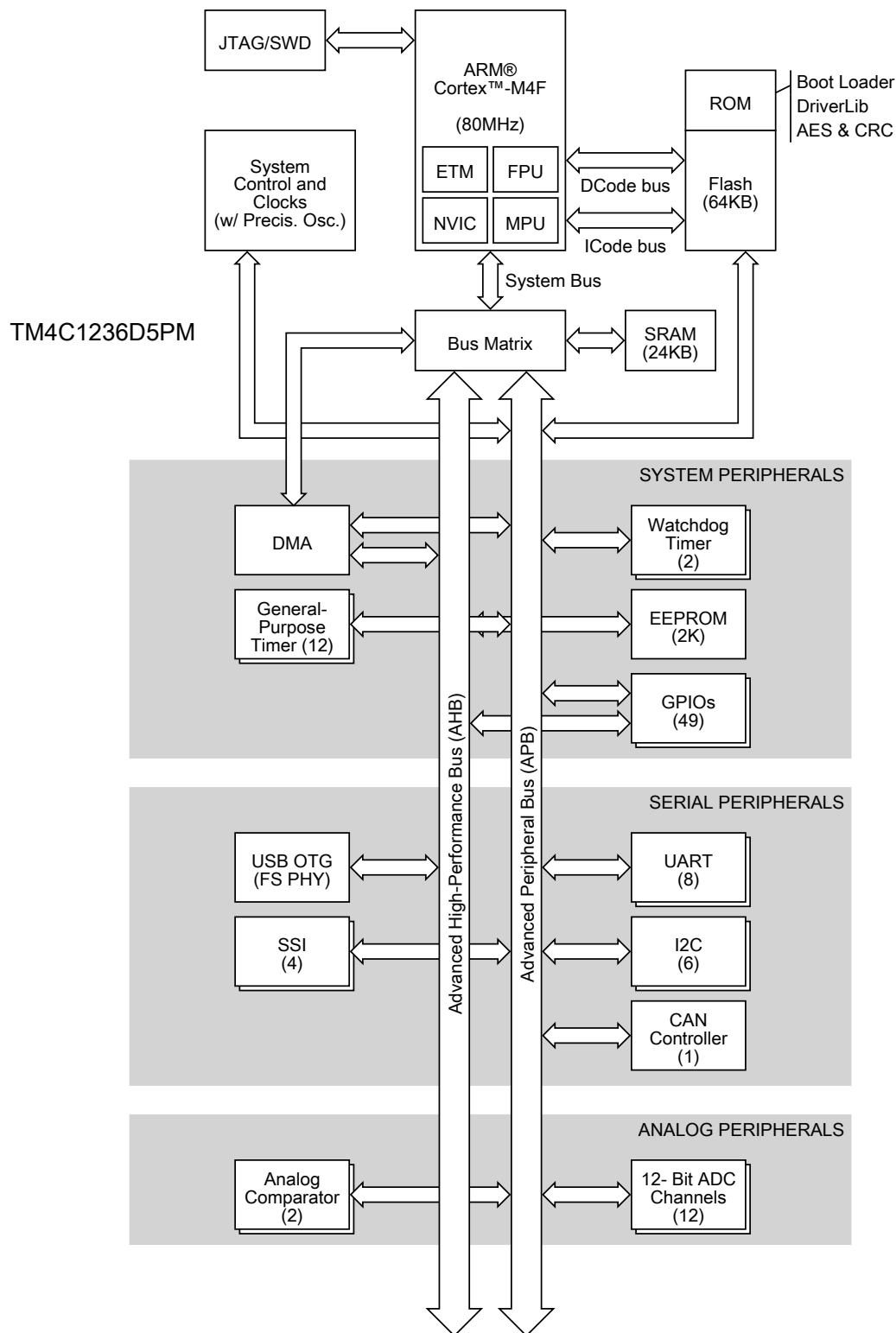
Figure 1-2. Tiva TM4C1236D5PM Microcontroller High-Level Block Diagram
