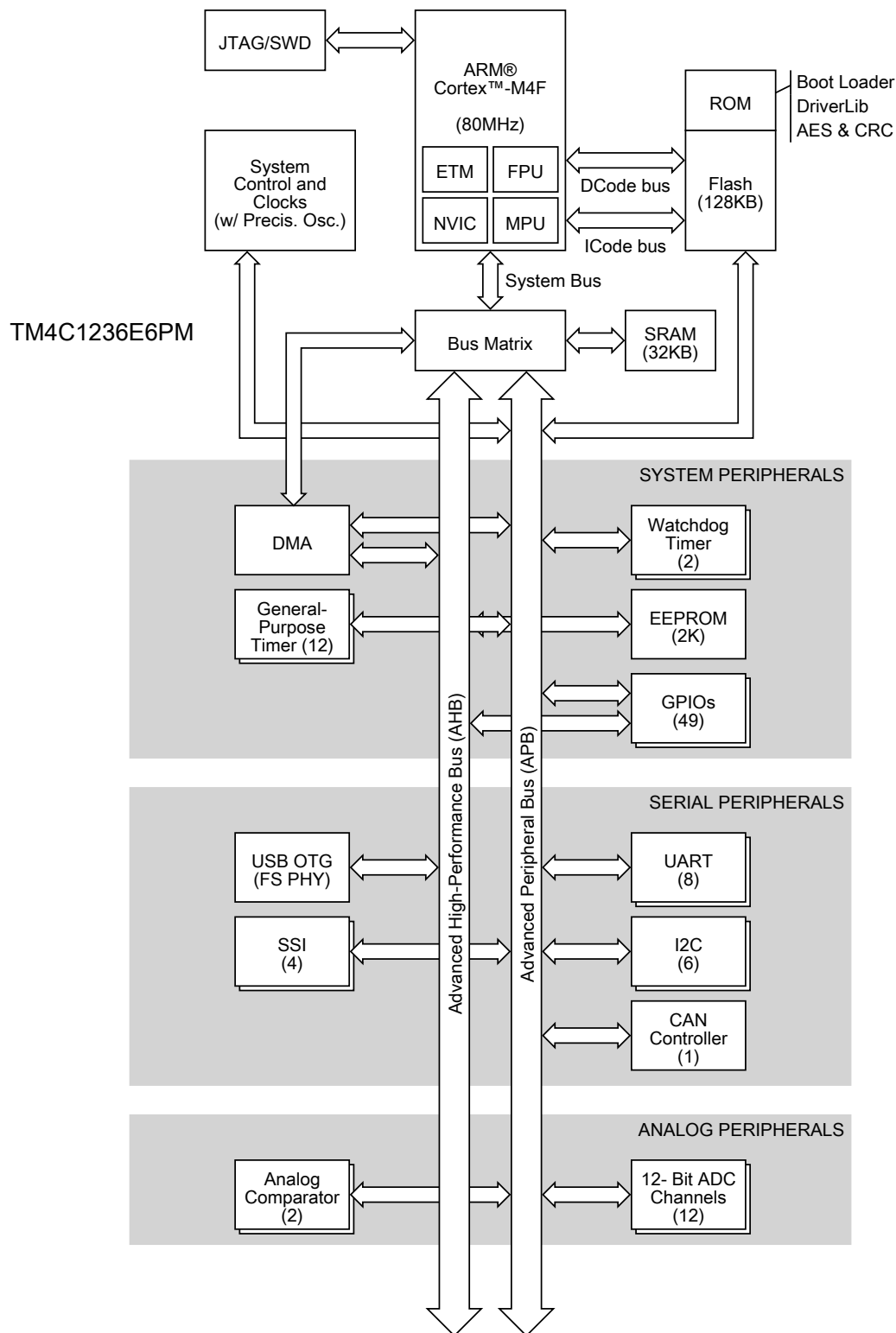
Figure 1-2. Tiva TM4C1236E6PM Microcontroller High-Level Block Diagram
