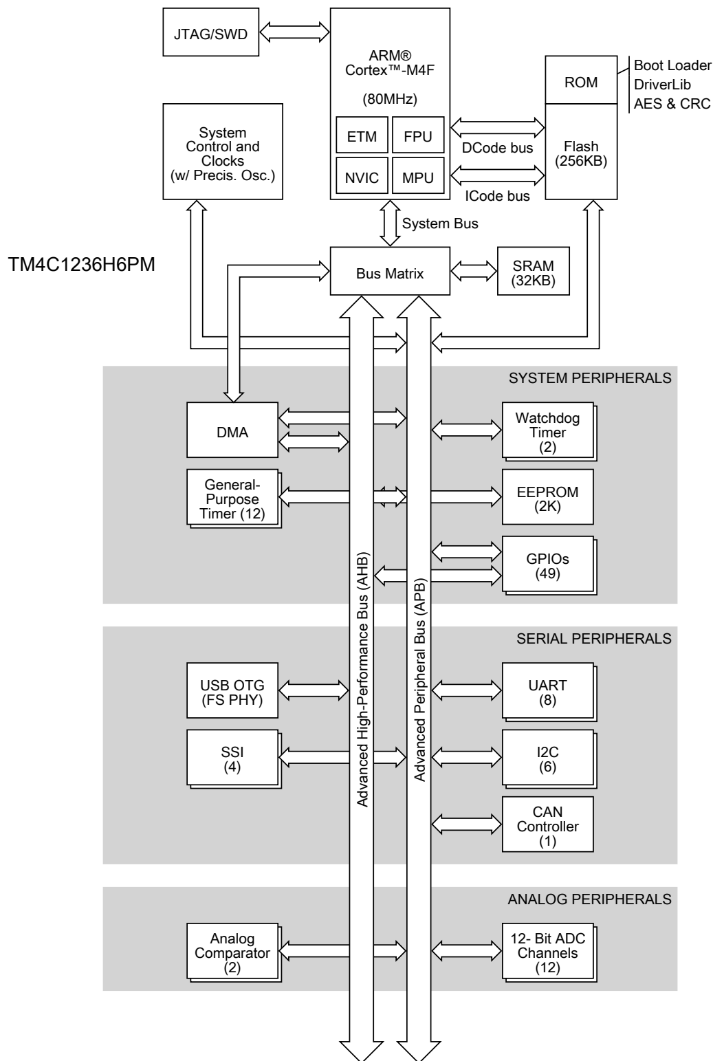
Figure 1-2. Tiva TM4C1236H6PM Microcontroller High-Level Block Diagram
