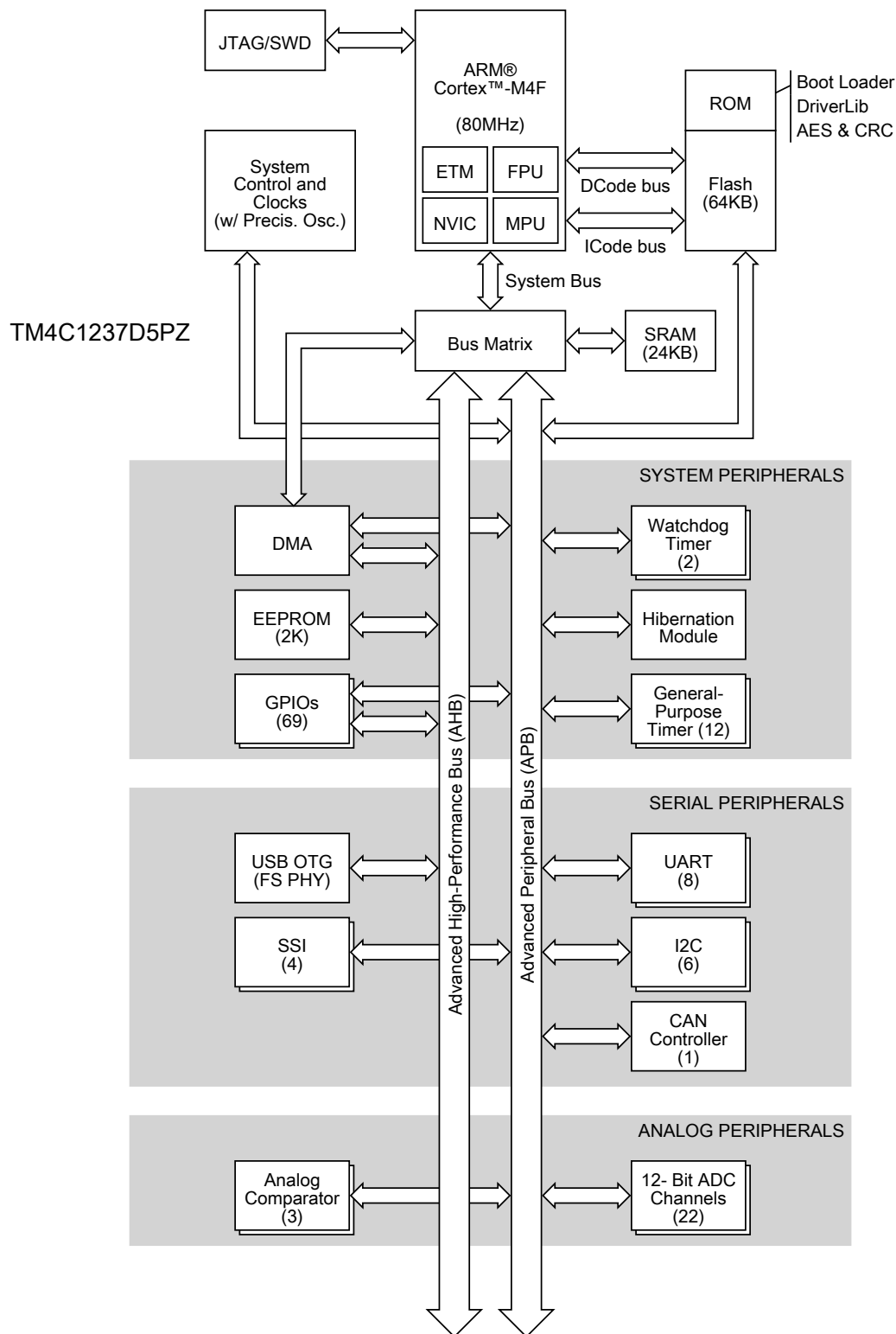
Figure 1-2. Tiva TM4C1237D5PZ Microcontroller High-Level Block Diagram
