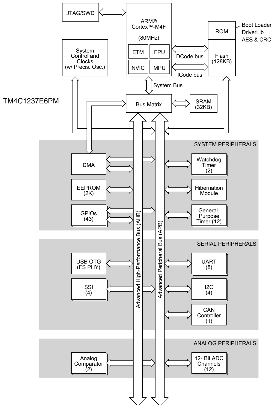
Figure 1-2. Tiva TM4C1237E6PM Microcontroller High-Level Block Diagram
