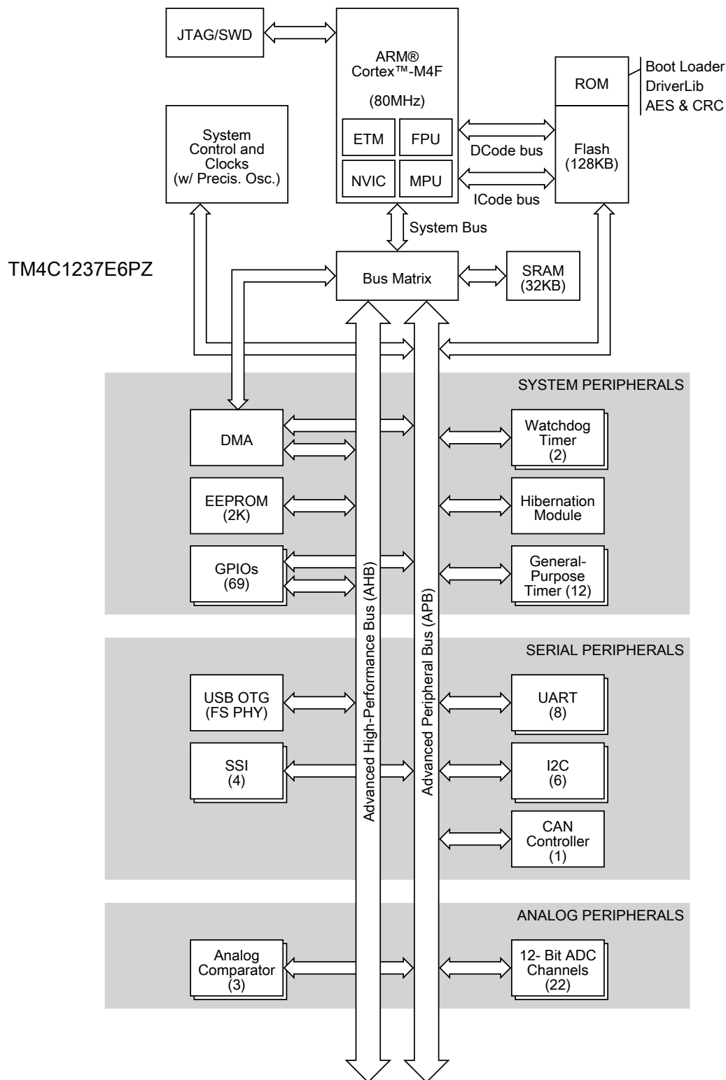
Figure 1-2. Tiva TM4C1237E6PZ Microcontroller High-Level Block Diagram
