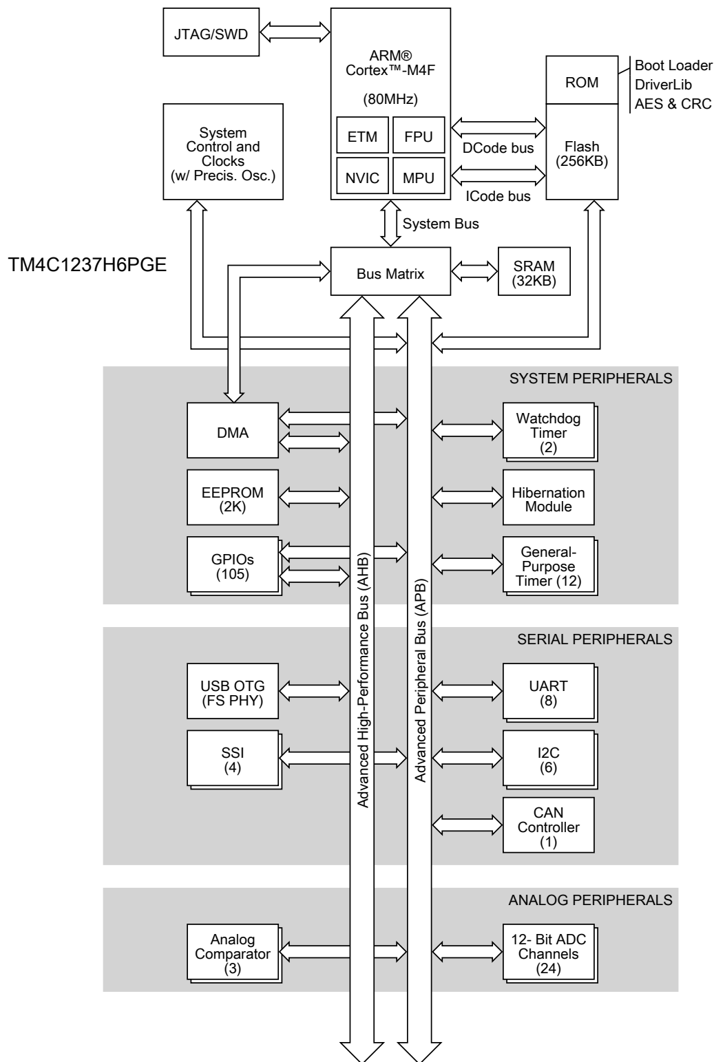
Figure 1-2. Tiva TM4C1237H6PGE Microcontroller High-Level Block Diagram
