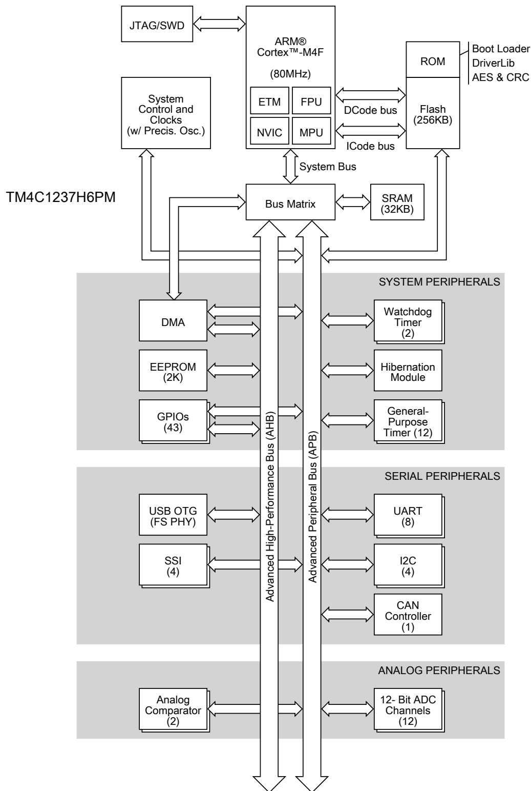
Figure 1-2. Tiva TM4C1237H6PM Microcontroller High-Level Block Diagram
