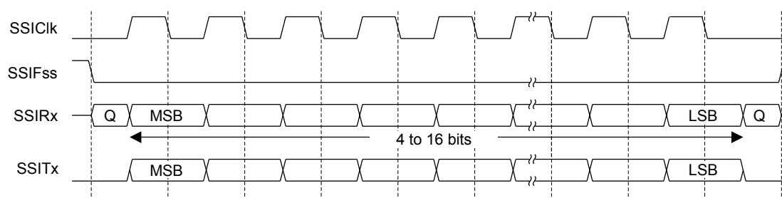
Figure 15-6. Freescale SPI Frame Format with SPO=0 and SPH=1
