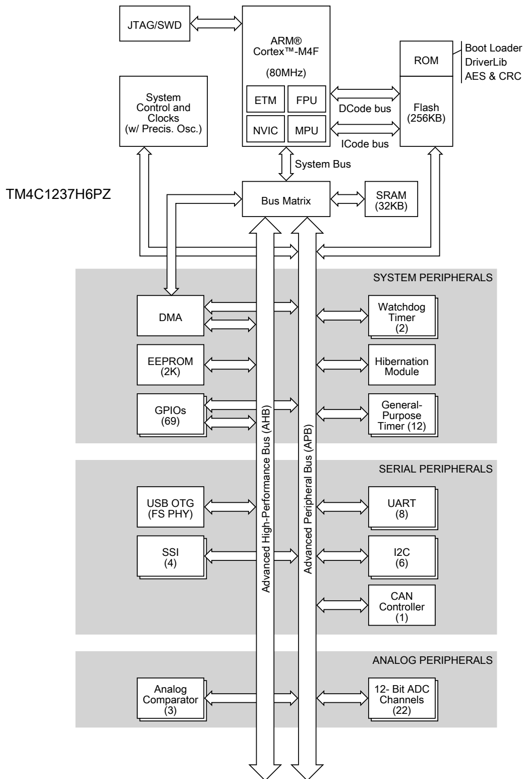
Figure 1-2. Tiva TM4C1237H6PZ Microcontroller High-Level Block Diagram
