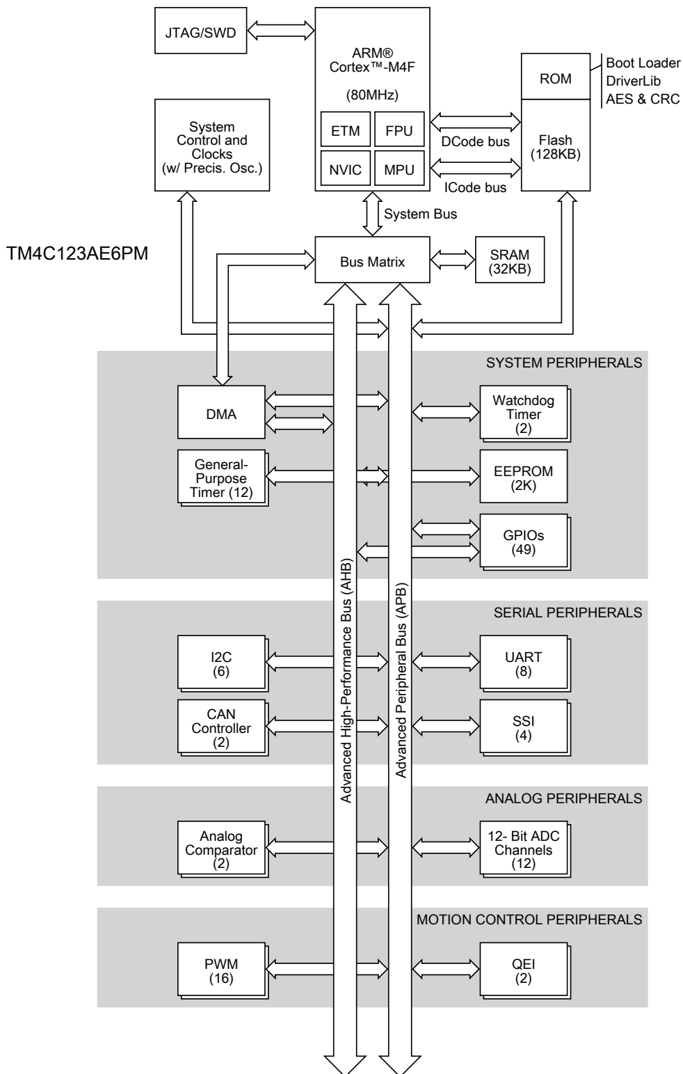
Figure 1-2. Tiva TM4C123AE6PM Microcontroller High-Level Block Diagram
