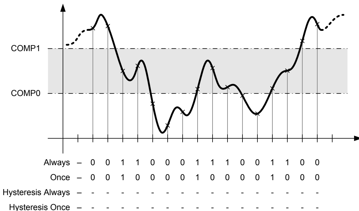
Figure 12-13. Mid-Band Operation (CIC=0x1 and/or CTC=0x1)
