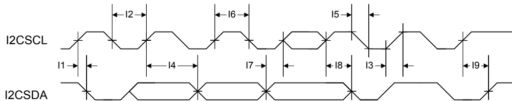
Figure 22-21. I 2 C Timing
