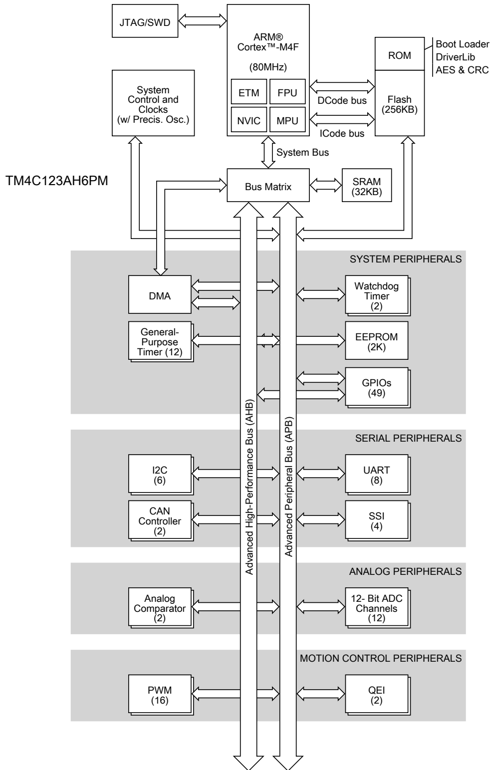
Figure 1-2. Tiva TM4C123AH6PM Microcontroller High-Level Block Diagram
