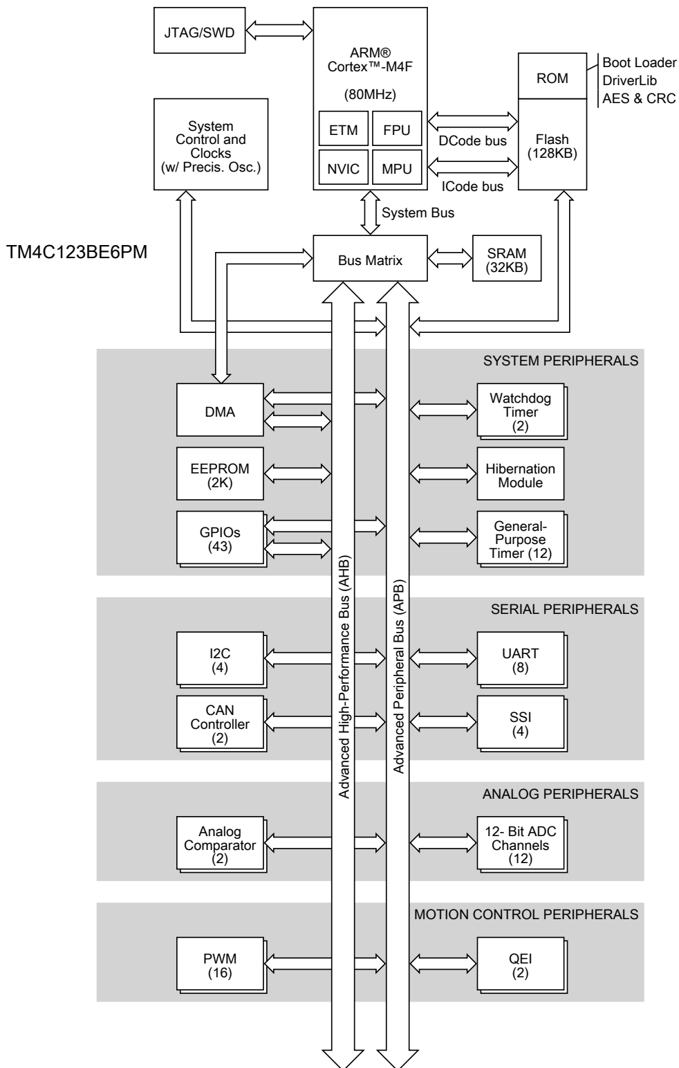
Figure 1-2. Tiva TM4C123BE6PM Microcontroller High-Level Block Diagram
