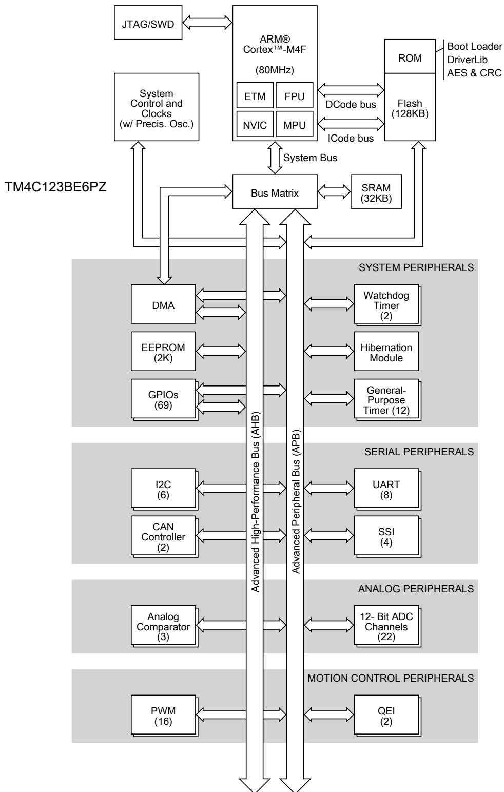
Figure 1-2. Tiva TM4C123BE6PZ Microcontroller High-Level Block Diagram
