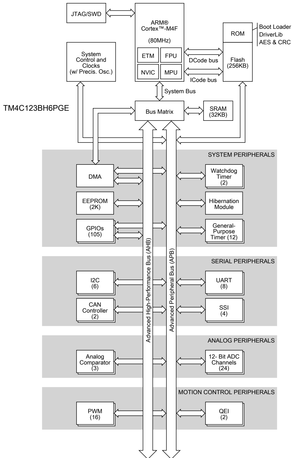
Figure 1-2. Tiva TM4C123BH6PGE Microcontroller High-Level Block Diagram
