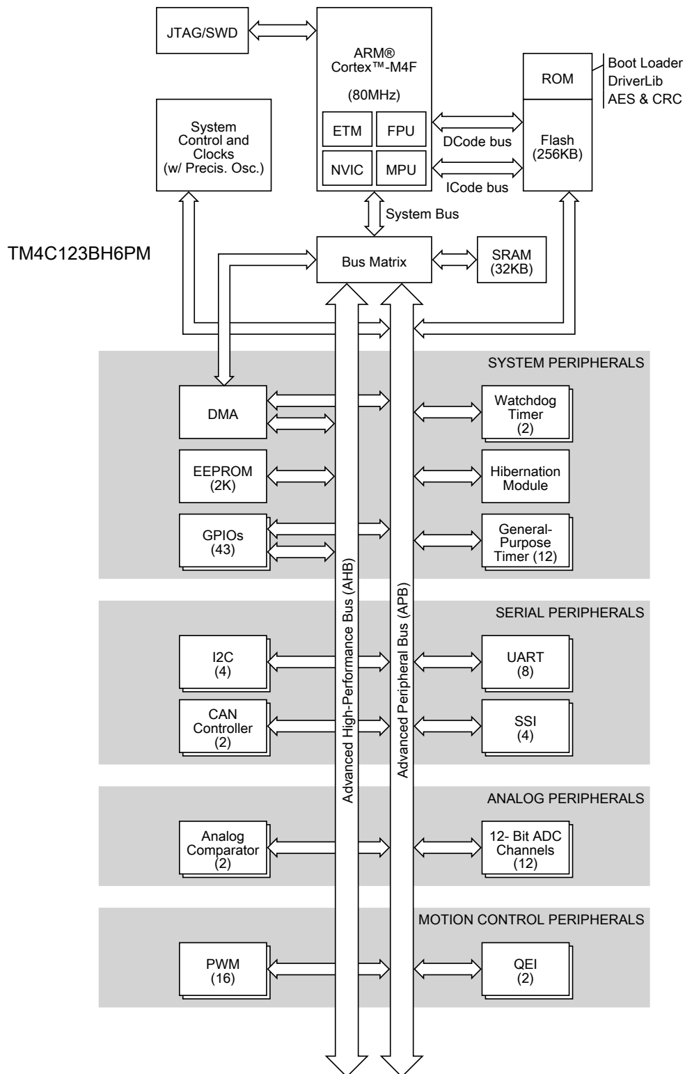
Figure 1-2. Tiva TM4C123BH6PM Microcontroller High-Level Block Diagram
