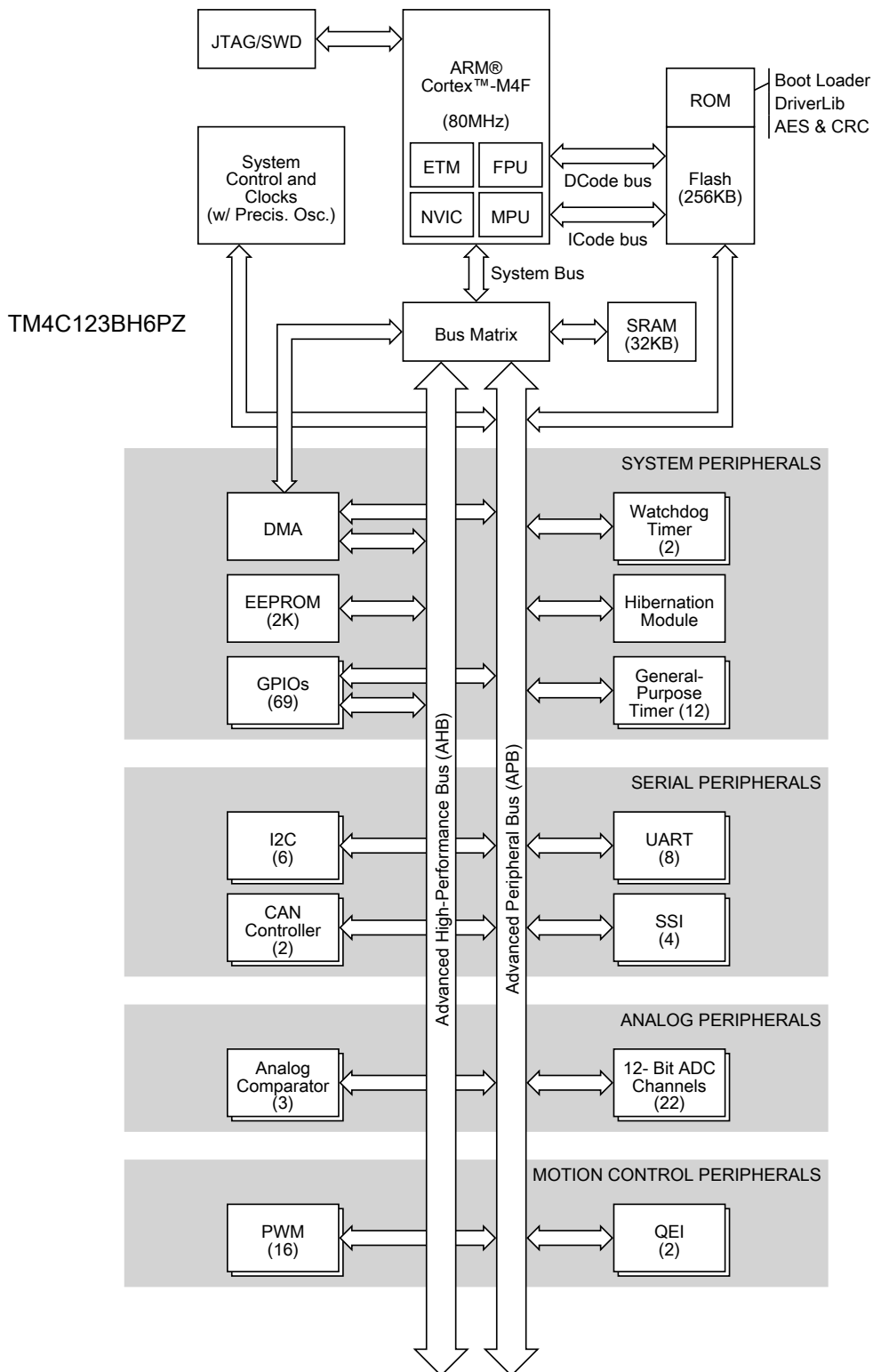
Figure 1-2. Tiva TM4C123BH6PZ Microcontroller High-Level Block Diagram
