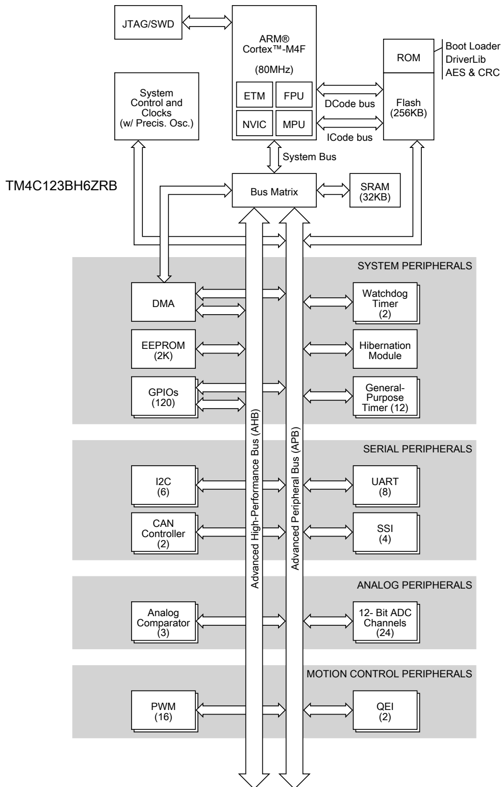
Figure 1-2. Tiva TM4C123BH6ZRB Microcontroller High-Level Block Diagram
