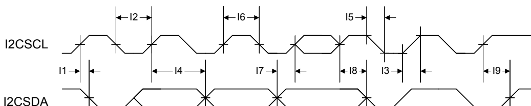
Figure 23-23. I 2 C Timing
