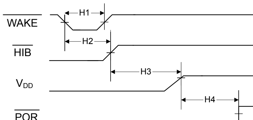
Figure 23-15. Hibernation Module Timing
