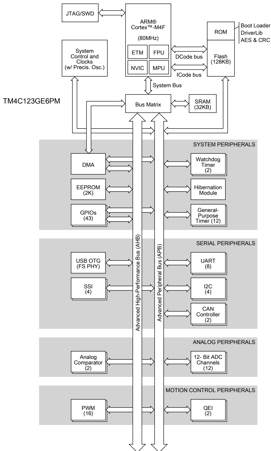
Figure 1-2. Tiva TM4C123GE6PM Microcontroller High-Level Block Diagram
