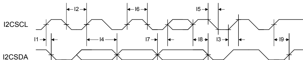
Figure 24-22. I 2 C Timing
