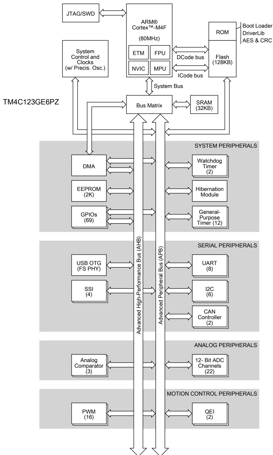
Figure 1-2. Tiva TM4C123GE6PZ Microcontroller High-Level Block Diagram
