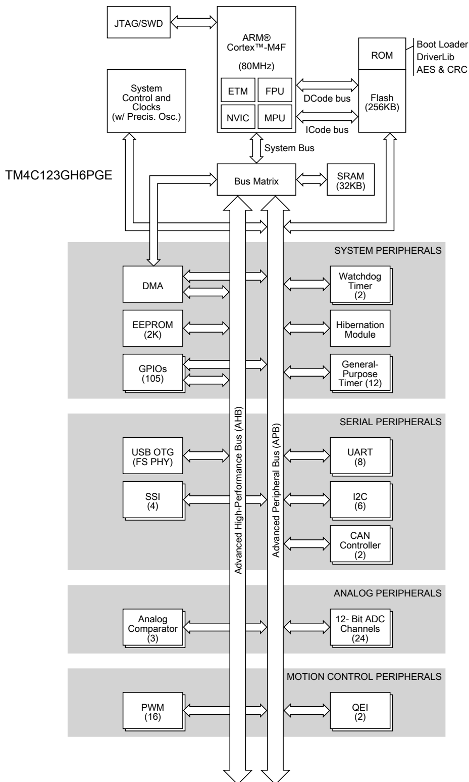
Figure 1-2. Tiva TM4C123GH6PGE Microcontroller High-Level Block Diagram
