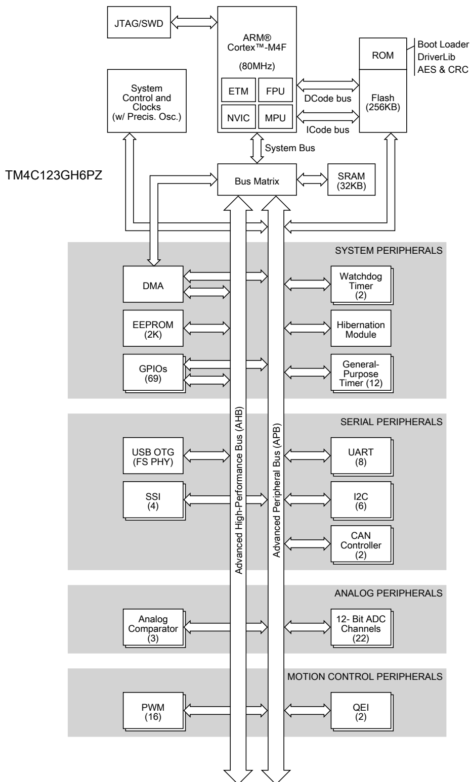
Figure 1-2. Tiva TM4C123GH6PZ Microcontroller High-Level Block Diagram
