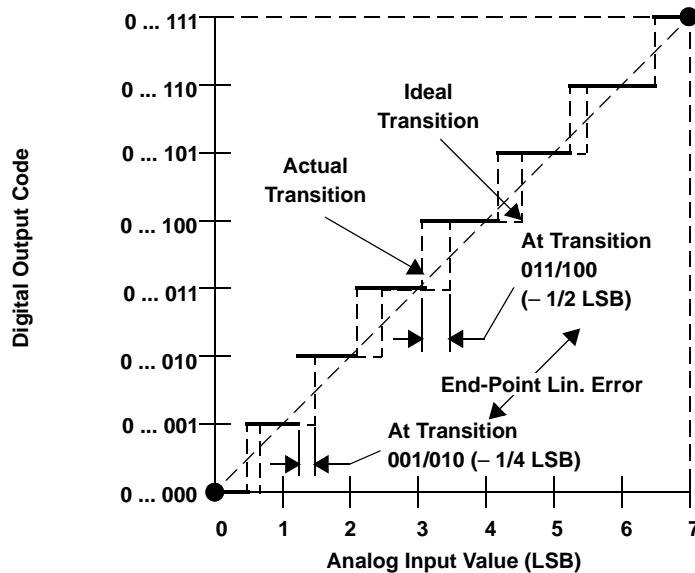
Figure 19. Integral Nonlinearity (INL) Error
