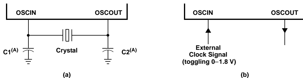
Figure 5. Crystal/Clock Connection
