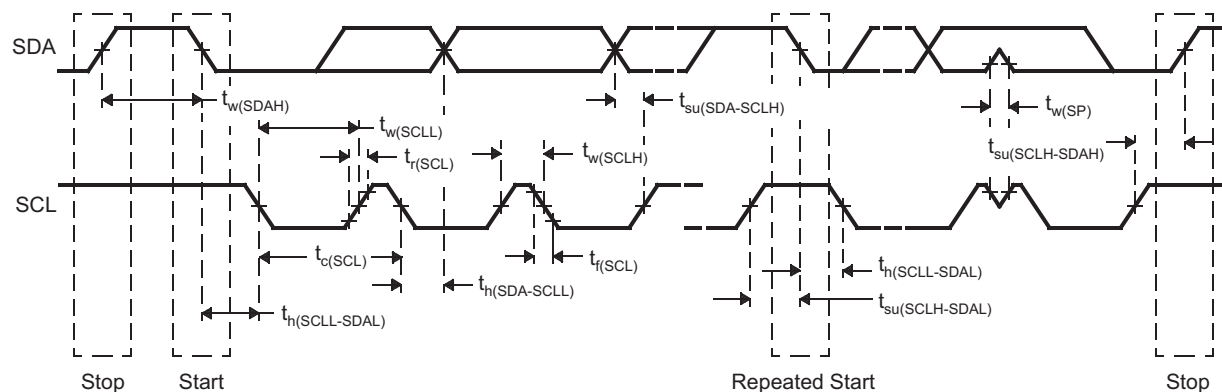
Figure 5-9. I2C Timings
