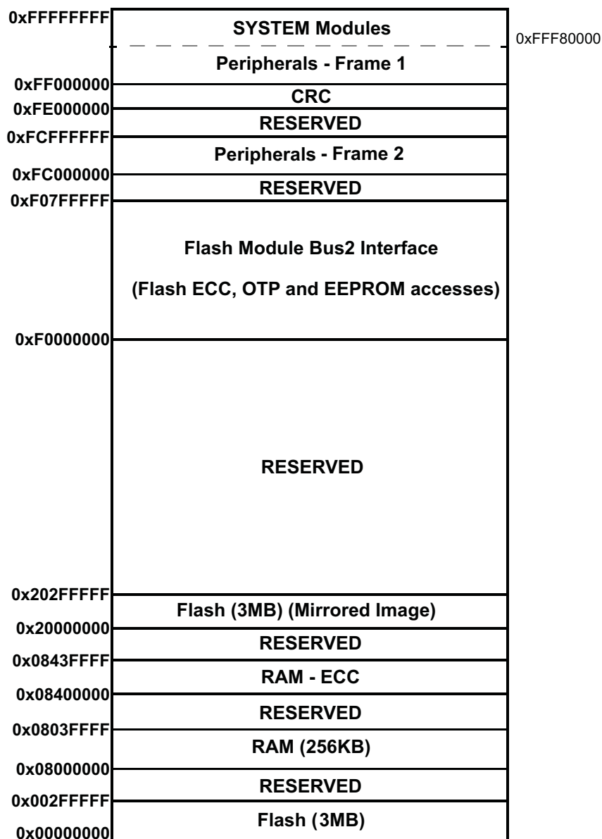
Figure 4-9. Memory Map
