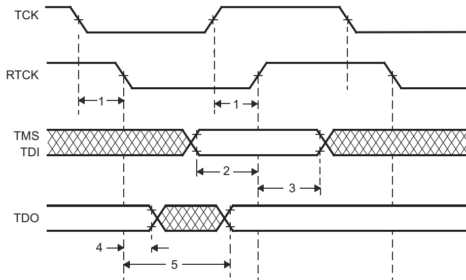
Figure 4-14. JTAG Timing
