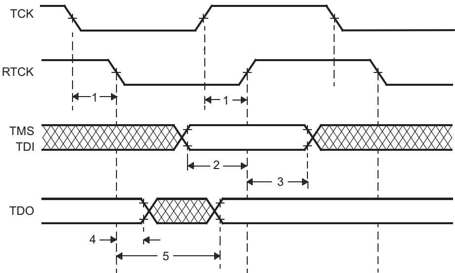
Figure 4-21. JTAG Timing
