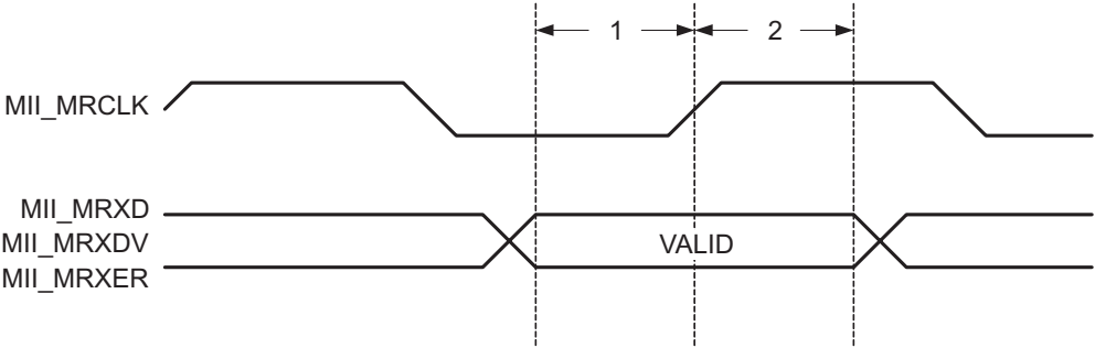
Figure 5-22. MII Receive Timing
