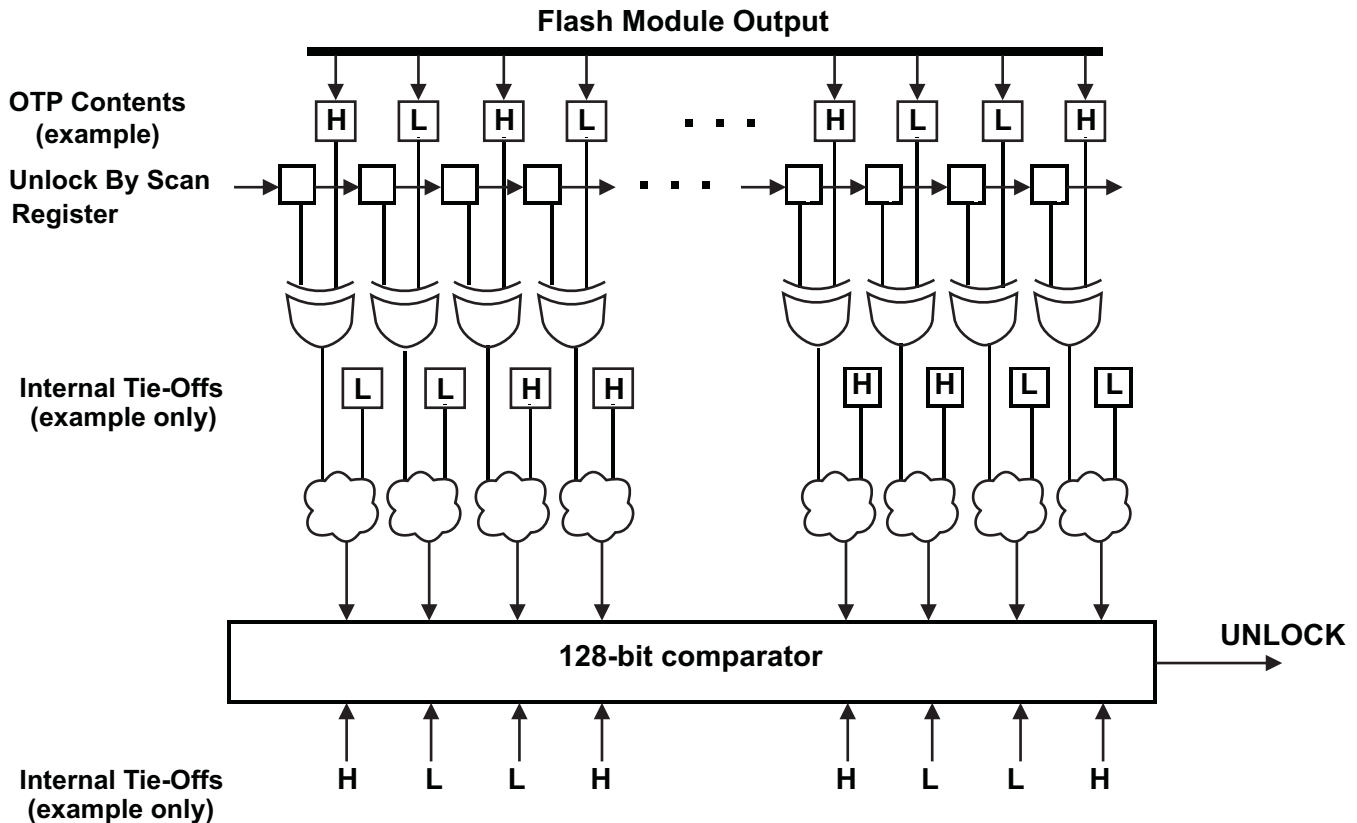
Figure 4-21. AJSM Unlock
