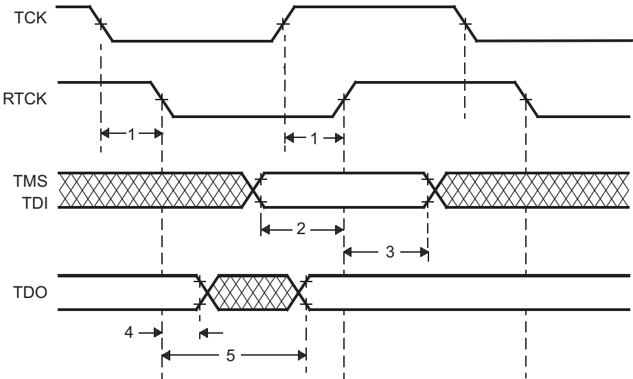
Figure 4-20. JTAG Timing
