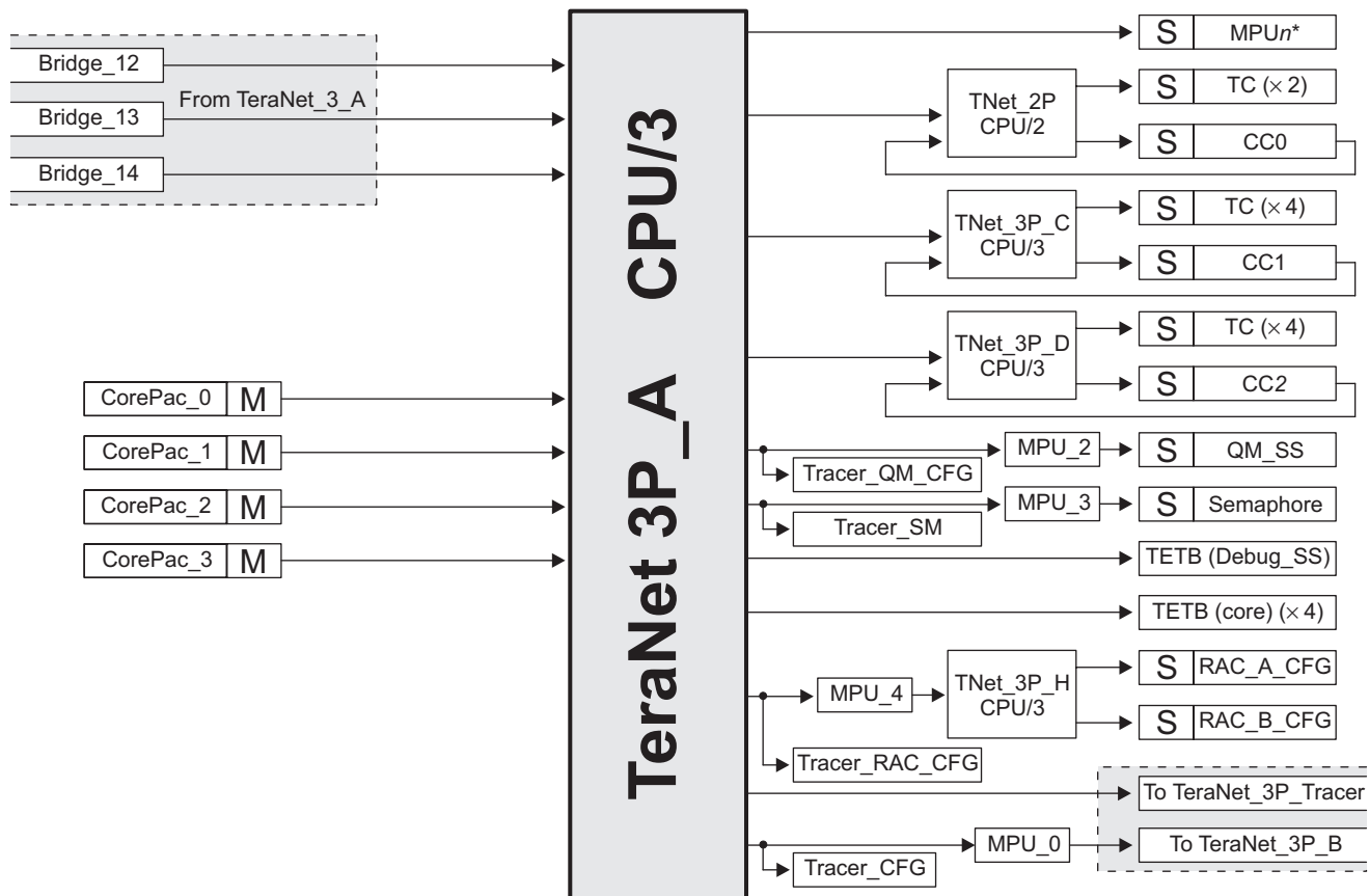
Figure 4-3 TeraNet 3P_A
