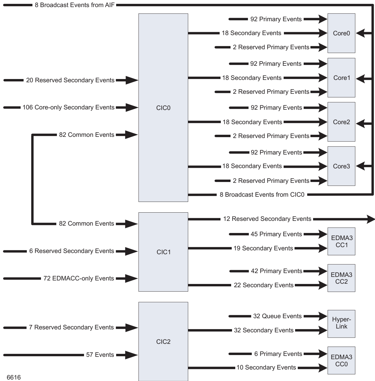
Figure 7-29 Interrupt Topology
