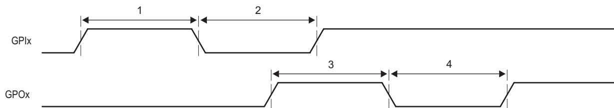
Figure 7-53 GPIO Timing
