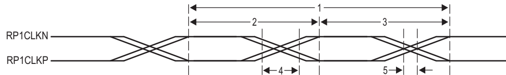
Figure 7-55 AIF2 RP1 Frame Synchronization Burst Timing
