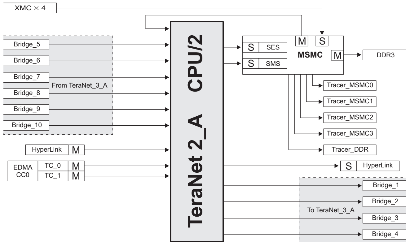
Figure 4-2 TeraNet 2A
