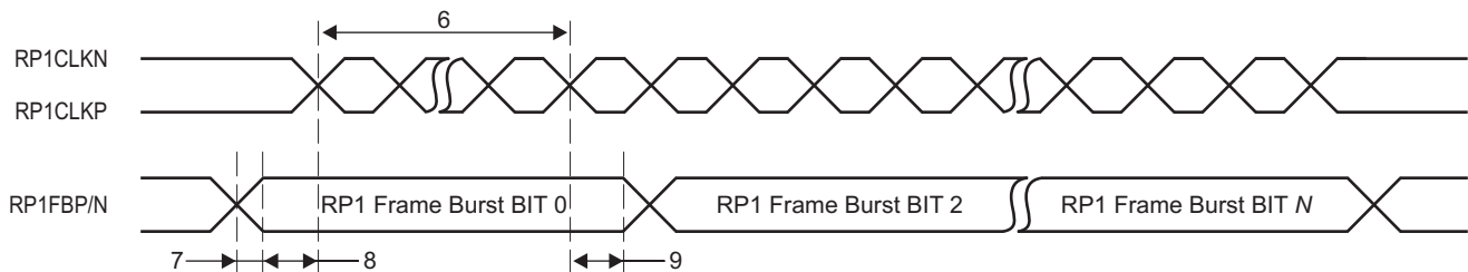
Figure 7-56 AIF2 Physical Layer Synchronization Pulse Timing
