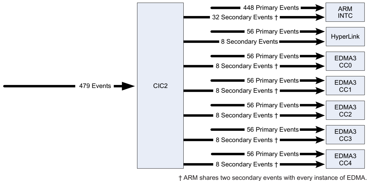
Figure 3-4 Interrupt Topology for AM5K2E04/02
