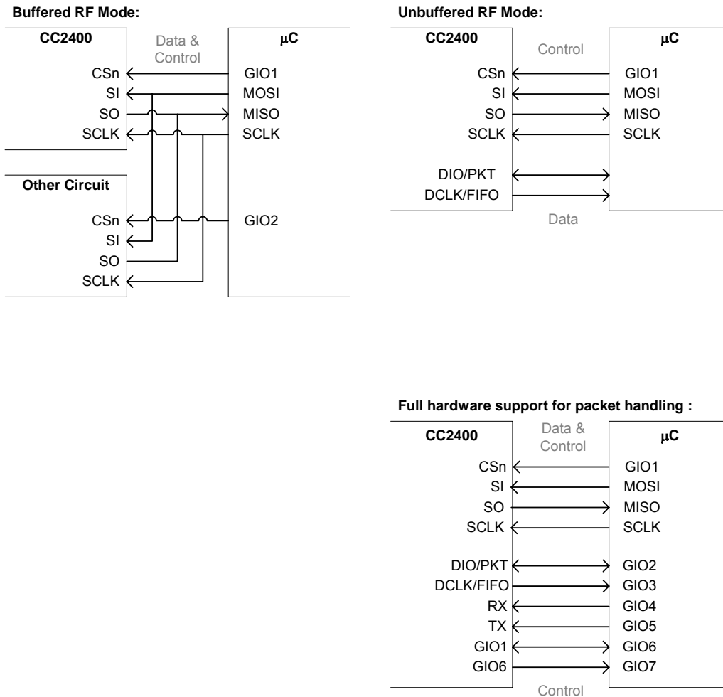
Figure 8. Microcontroller interface
